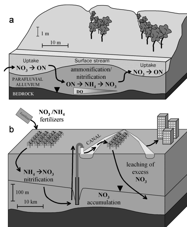
Figure 5. Conceptual model of how surface-subsurface interactions determine nitrate ( \text{NO}_3^- ) availability in Sycamore Creek (a) and the Indian Bend Wash (IBW) ecosystem (b). The processes of assimilation, ammonification-nitrification, and hydrologic exchange determine nitrogen (N) dynamics in both systems, but the scales at which these processes operate differ markedly. Cycling of N in Sycamore Creek is rapid and tightly coupled to biotic drivers, and it occurs over short spatial scales. Conversely, N cycling in the IBW is slow and dominated by human inputs, and it is characterized by long lag times between the leaching of N into groundwater and its return to surface ecosystems. Further, groundwater pumping and canals establish spatial connections between distant, formerly isolated patches in the IBW. Finally, drivers of hydrologic exchange in the two ecosystems are different, with physical processes forcing movement of water between surface and subsurface systems in Sycamore Creek, whereas human actions connect groundwater with surface flows in the IBW. Abbreviations: DO, dissolved oxygen; \text{NH}_4^+ , ammonium; ON, organic N.
